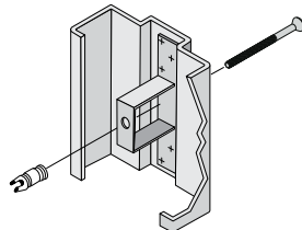
MASONRY WIRE ANCHOR
